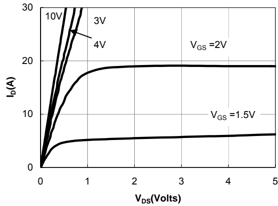
Figure 1: On-Regions Characteristics
